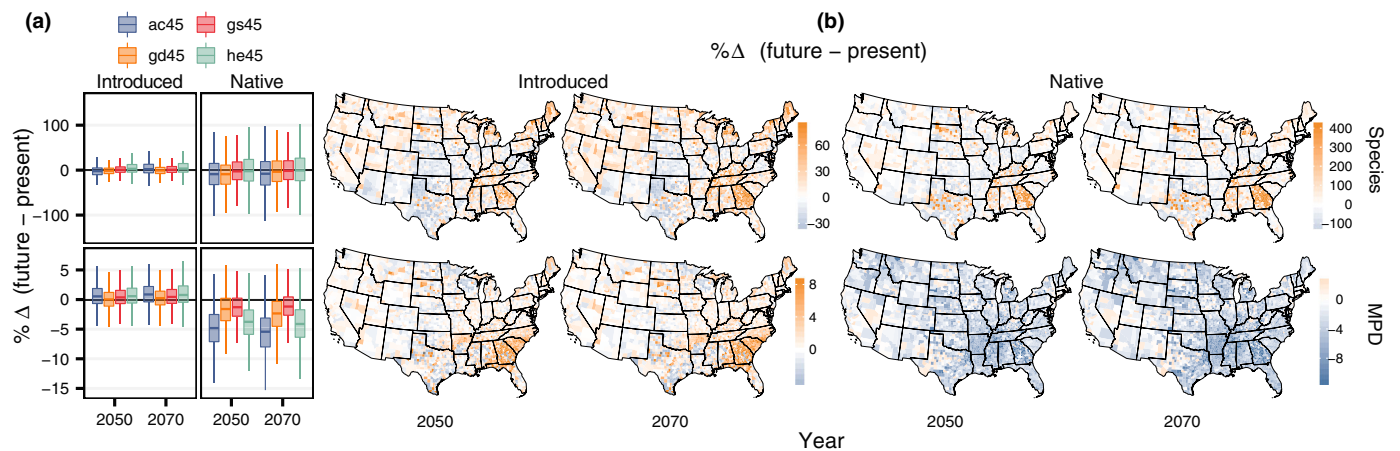
Fig. 2 Predicted changes in native vs nonnative introduced species richness and mean phylogenetic diversity in 2050 and 2070 relative to current values under RCP4.5. (a) Boxplots depict the percentage difference between predicted future values for 2050/2070 and present day observed values, for each of four different general circulation models (ACCESS1-0 (ac), GISS-E2-R (gs), GFDL-ESM2G (gd) and HadGEM2-ES (he)) and two response variables (species, MPD). (b) Choropleth maps illustrate the average percentage difference over four different general circulation models (ACCESS1-0 (ac), GISS-E2-R (gs), GFDL-ESM2G (gd), and HadGEM2-ES (he)) between predicted future values for 2050 and 2070 and present day observed values, for each of two response variables (species, MPD). The color gradient indicates increases (orange) and decreases (blue) in each metric.
