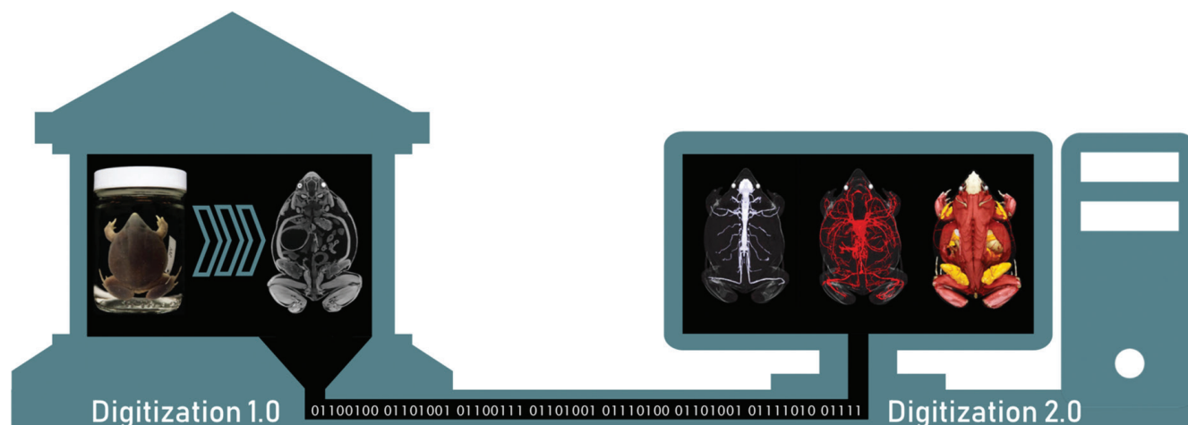
Figure 2. An example pipeline to highlight the value and complementarity of Digitization 1.0 and 2.0. The African pig-nosed frog (genus Hemisus ) shown was collected during recent field research in Angola. In addition to metadata from the collection event, a series of X-ray images (tomograms) were created using diffusible iodine-based contrast-enhanced computed tomography (diceCT) directly from the voucher specimen within an NHC (Digitization 1.0). This three-dimensional digital data (e.g., CT data) generated during Digitization 1.0 can be digitally dissected and manipulated by researchers or citizen scientists anywhere on the globe to highlight the frog's nervous, circulatory, and muscular systems (Digitization 2.0).
